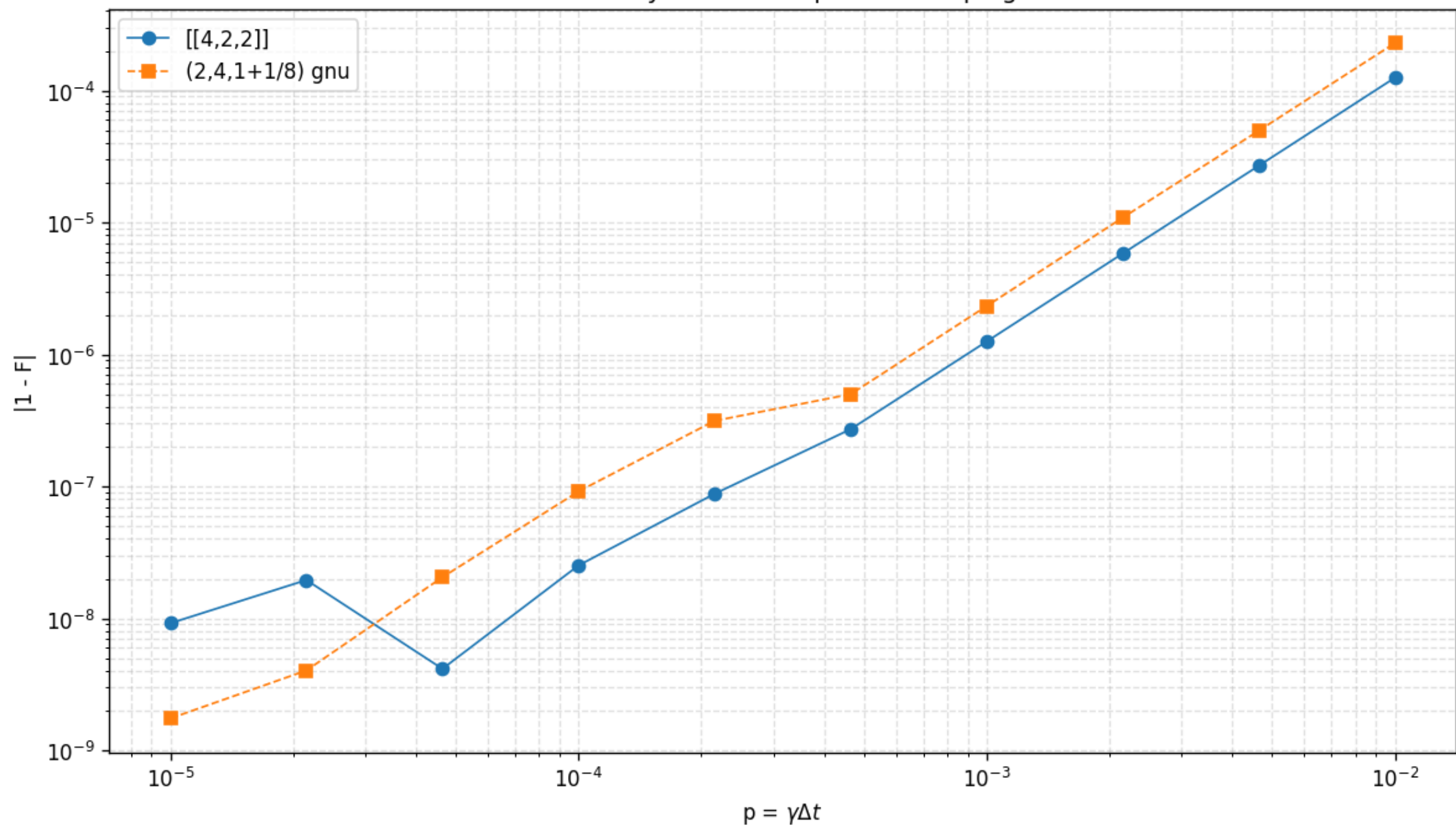
Global symmetric amplitude damping
